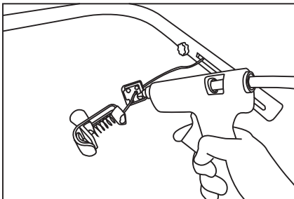
12. Apply glue inside the hook cover to make it stick to the hook.
