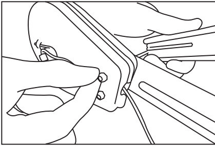
6. Mount the M4 x 35 screw. When the screw is through the nut it's perfect, otherwise the cover can bend.
